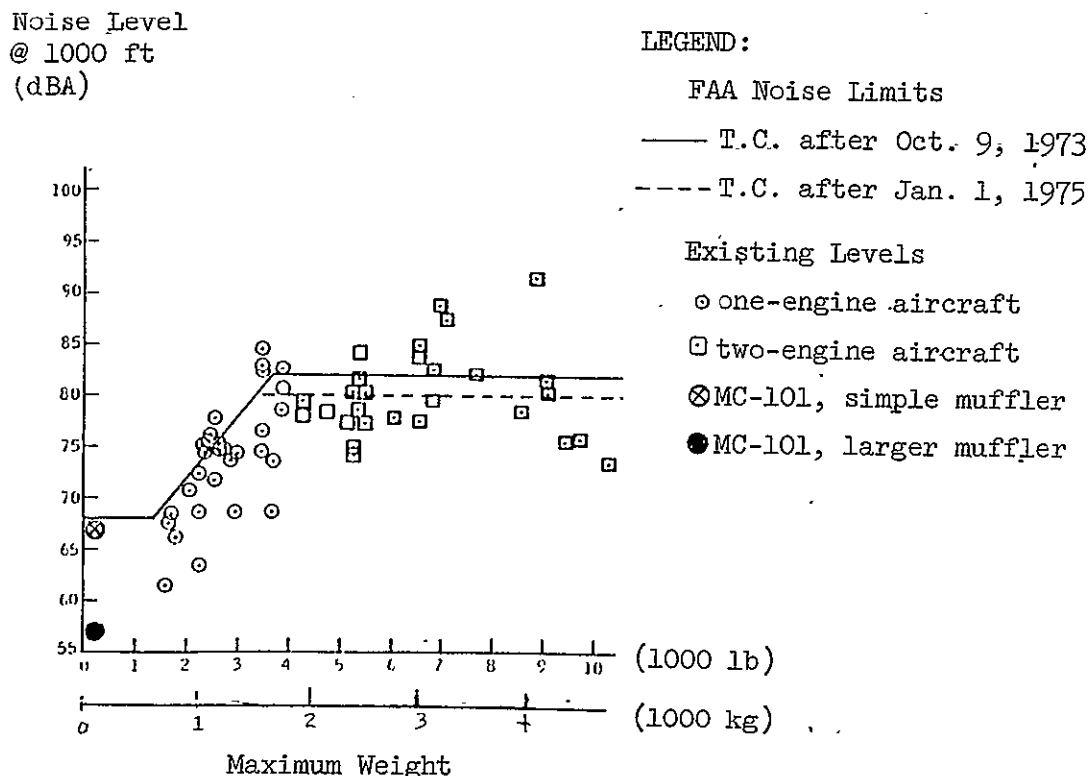
FIGURE 14 FAA NOISE LIMITS, WITH EXISTING AIRCRAFT COMPARED
