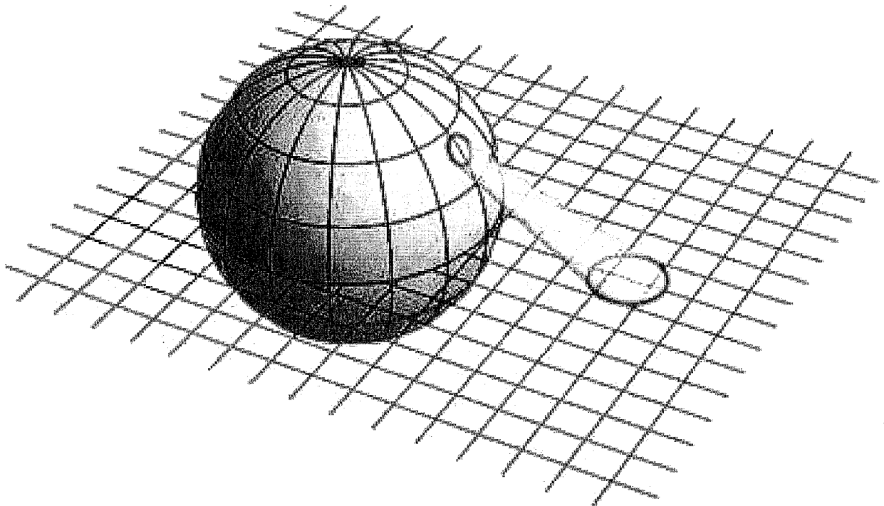
Figure 19. Stereographic Projection
