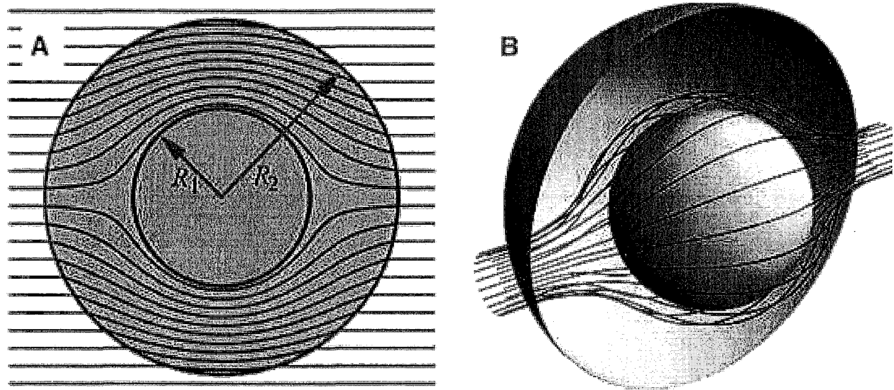
Figure 6. Cloaking Shell 6
